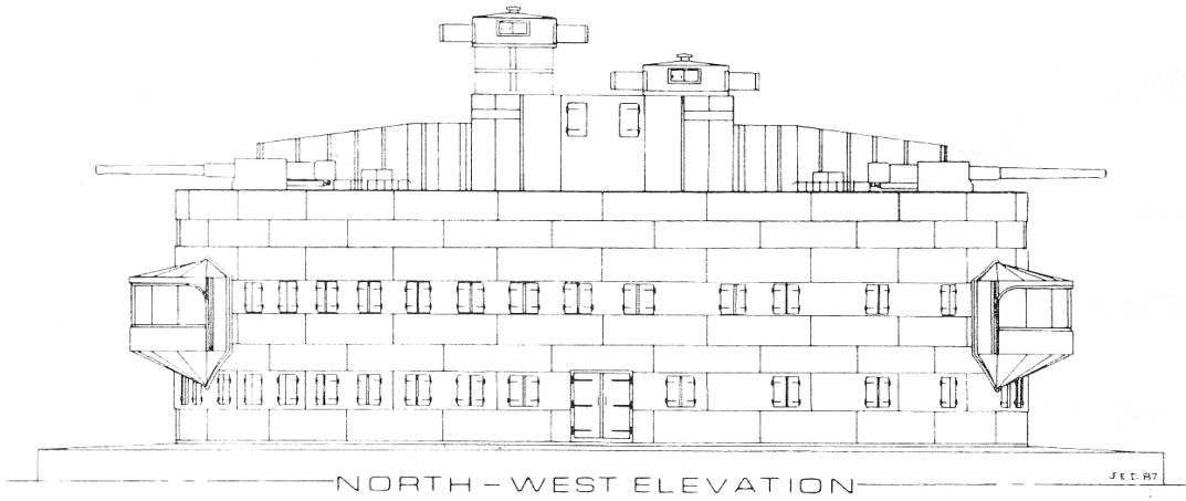
Bull Sand Fort, planned elevations, 1918
